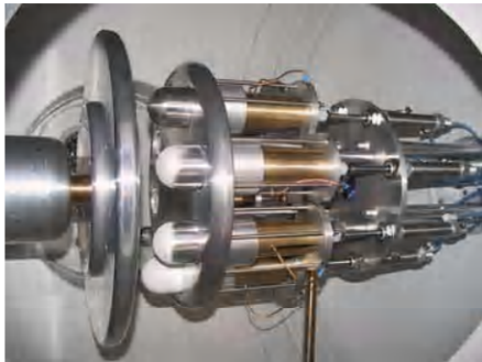
Figure 2: Pneumatically controlled revolver assembly for investigation of first breakdown
