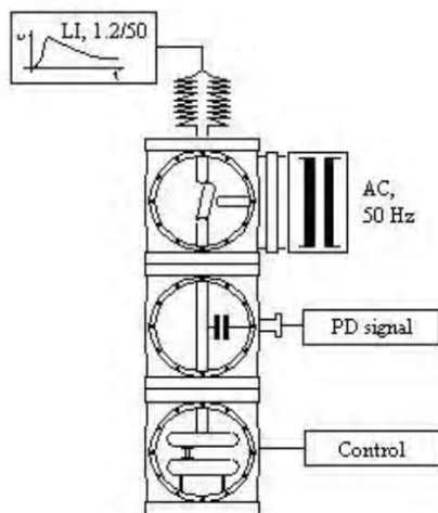
Fig.2 Test setup
