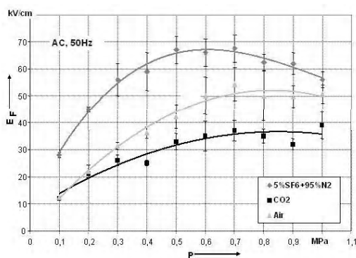
Fig.9 Flashover field strengths in compressed air, CO 2 and 5%SF 6 +95%N 2 under AC stress with particle contamination vs. pressure
