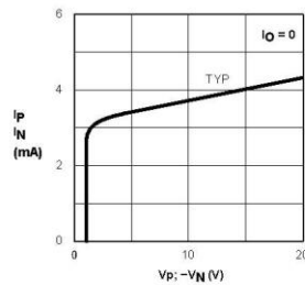
Figure 8. Supply Current
