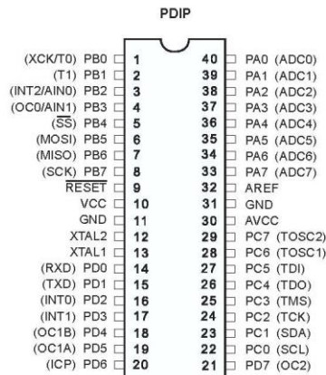
Figure 1. Pinouts ATmega16
