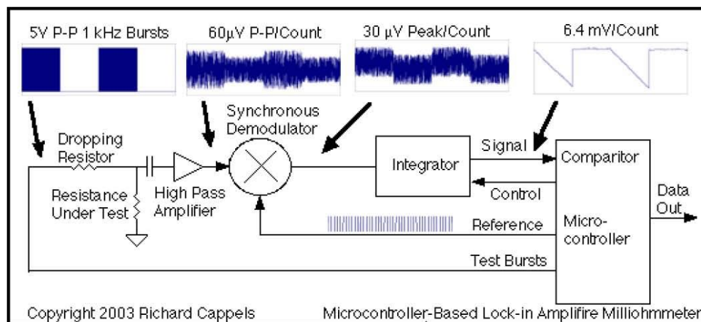
figure 1 The lock-in amplifier detects and integrates bursts of 1 kHz pulses that result from the IR drop across the
