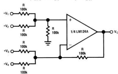
DC Summing Amplifier (V IN s ≥ 0 V DC and V O ≥ V DC )
