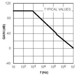
Figure 2. Open-Loop Frequency Response
