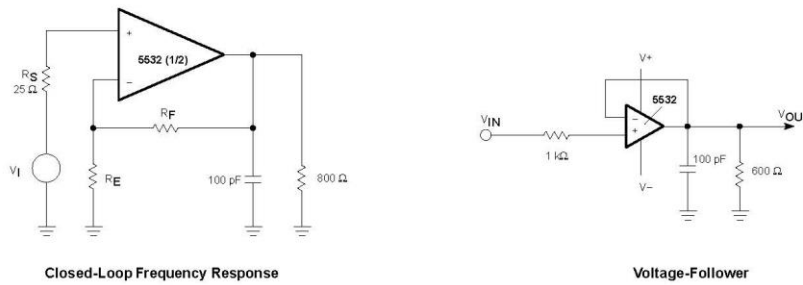
Figure 10. Test Circuits
