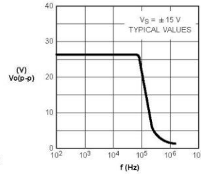
Figure 4. Large-Signal Frequency Response
