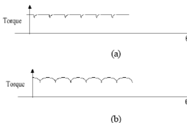
Fig. 6. Torque ripple in (a) rectangular and (b) sinusoidal controlled BLDC motor.
