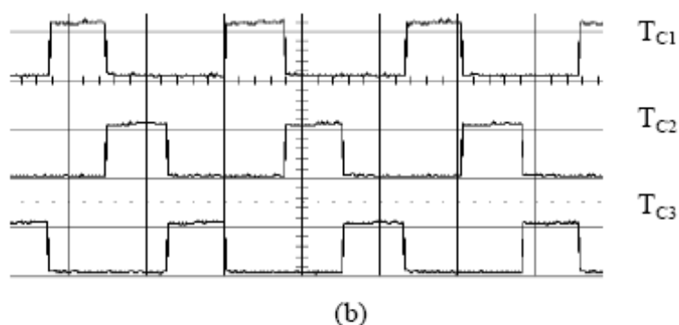
Fig. 14. Gating Signals for (a) Rectifier and (b) Chopper
