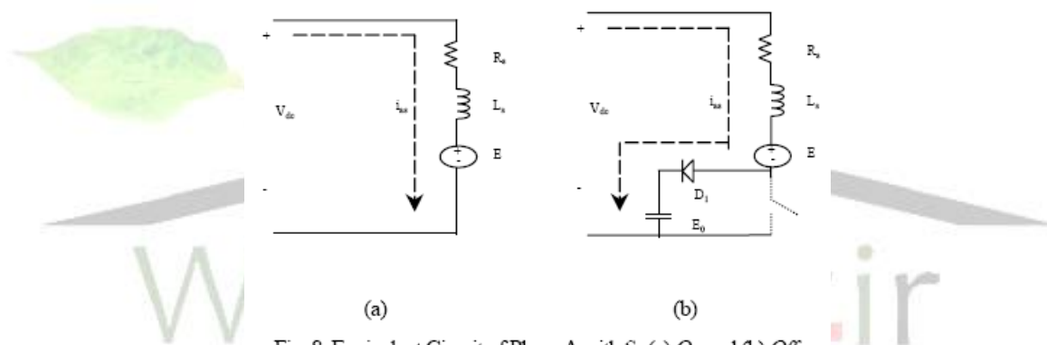
Fig. 8. Equivalent Circuit of Phase A with S 1 (a) On and (b) Off
