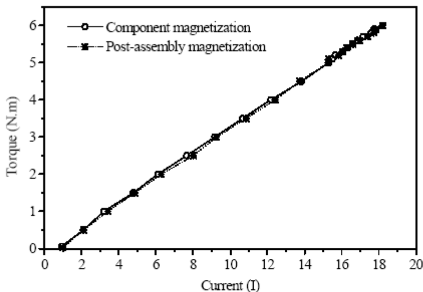
Fig. 9. Measured torque vs. current curves.
