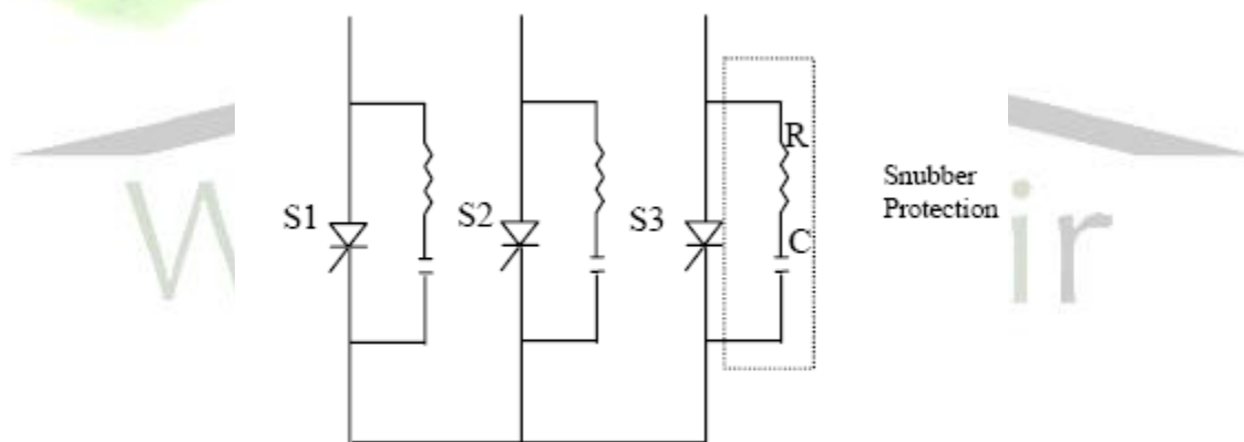
Fig. 11. Snubber Circuits for Thyristors
