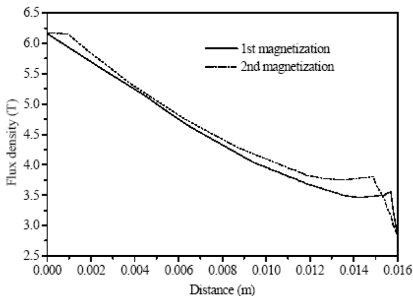
Fig. 4. Flux density vs. distance when slot current is 1.5 \times 10^5 \text{ A} .
