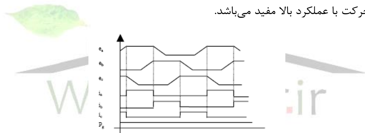
Fig. 5. Trapezoidal EMF and Square wave Current
