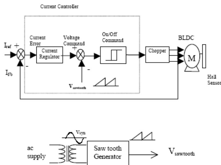
Fig. 4. Current Loop Block Diagram
