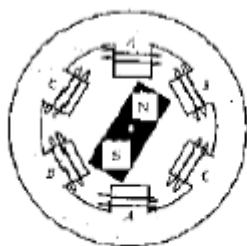
3-phase motor with permanent magnet rotor.
