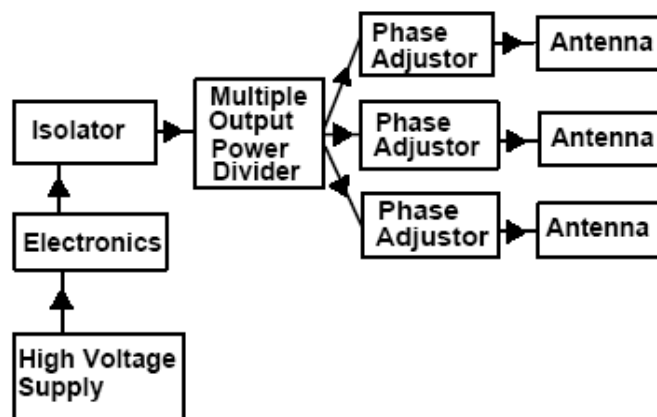
Fig. 4. Microwave power transmission system using electron tubes
