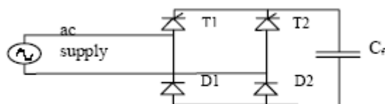
Fig. 3 Full-Wave Half Controlled Rectifier
