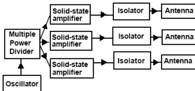
Fig. 5. Microwave power transmission system using semiconductors
