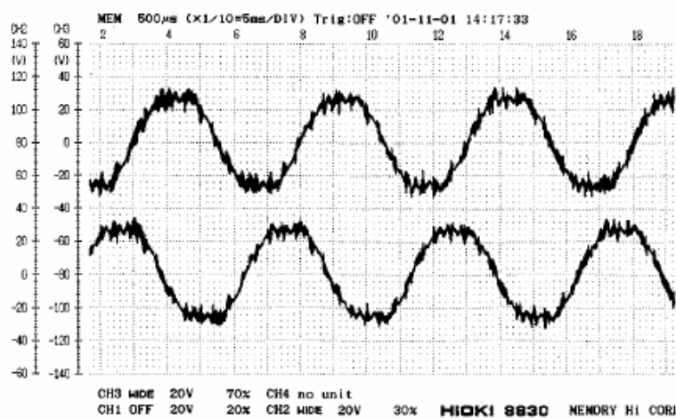
Fig. 8. Measured BEMF curve of post-assembly-magnetization motor.
